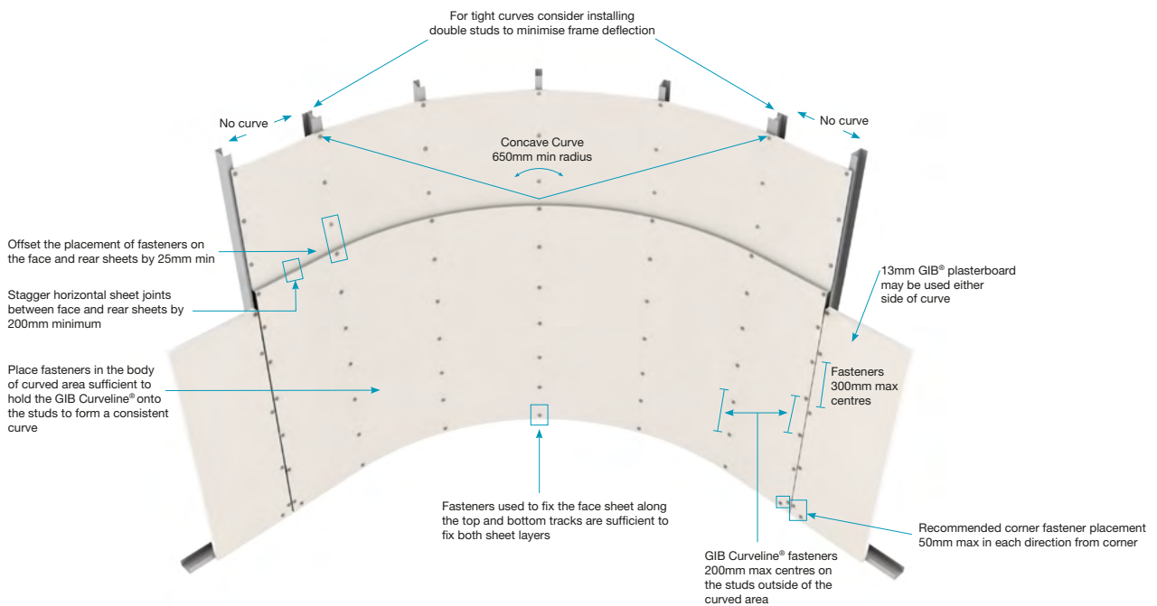
Figure 5: Concave Curved - Vertical Sheet Fixing
