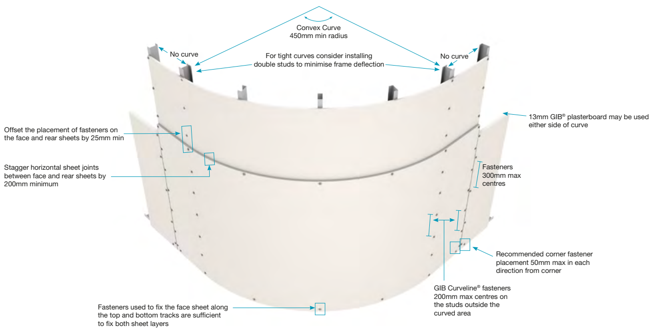
Figure 6: Convex Curved - Horizontal Sheet Fixing
