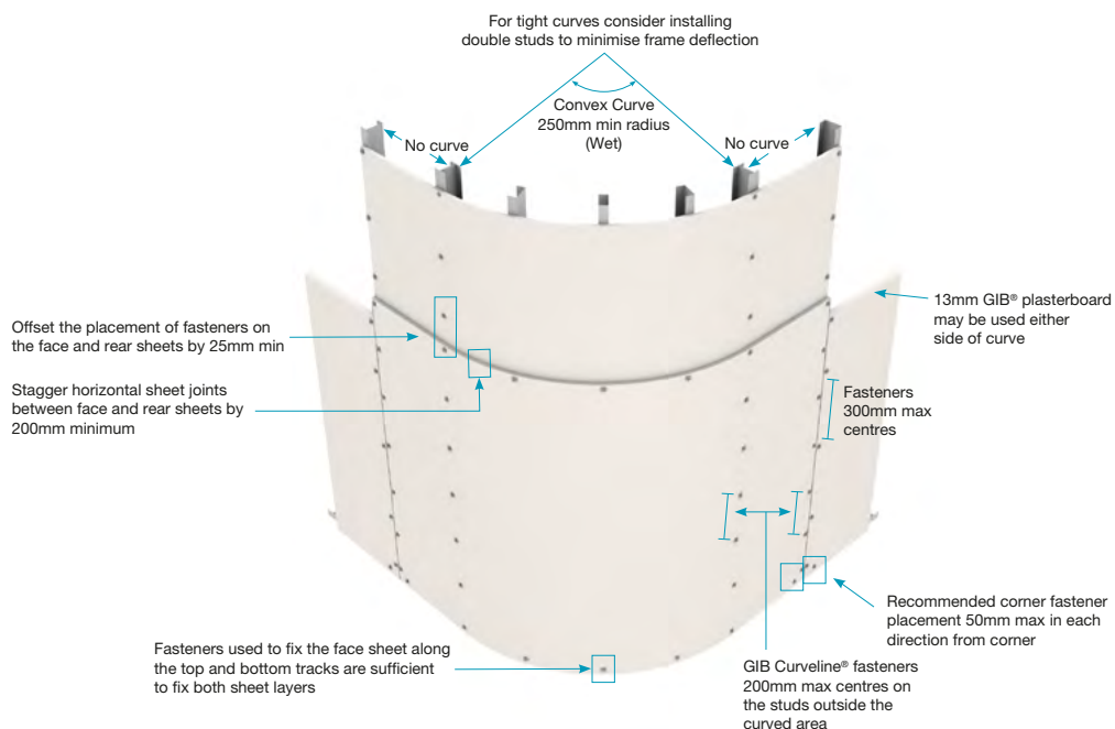
Figure 7: Convex Curved - Vertical Sheet Fixing
